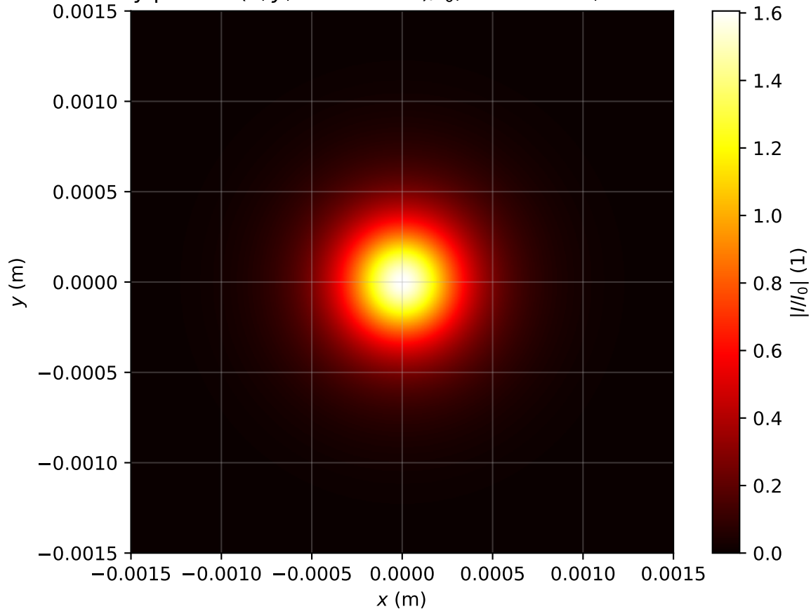
Intensity profile I(x, y, z = 1.115m)/I_0 , Pin=1.0Pcr, artificial time
